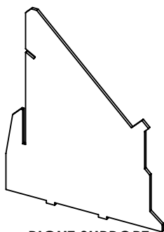
RIGHT SUPPORT (1 pc)
